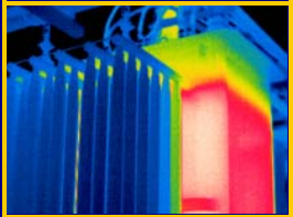
Cold Cooling Fins Due to Low Oil in Transformer
