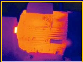
Internal Winding Problem in Motor
